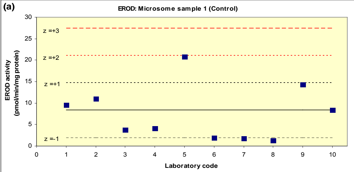
Figure 1 (a-i): EROD activity reported by each laboratory from prepared liver microsome samples of the S. maximus . Solid line represents overall mean, dotted lines denote the appropriate Z score values. Circled data points denote excluded outliers based on Dixon's Q-test at 95% CL.
